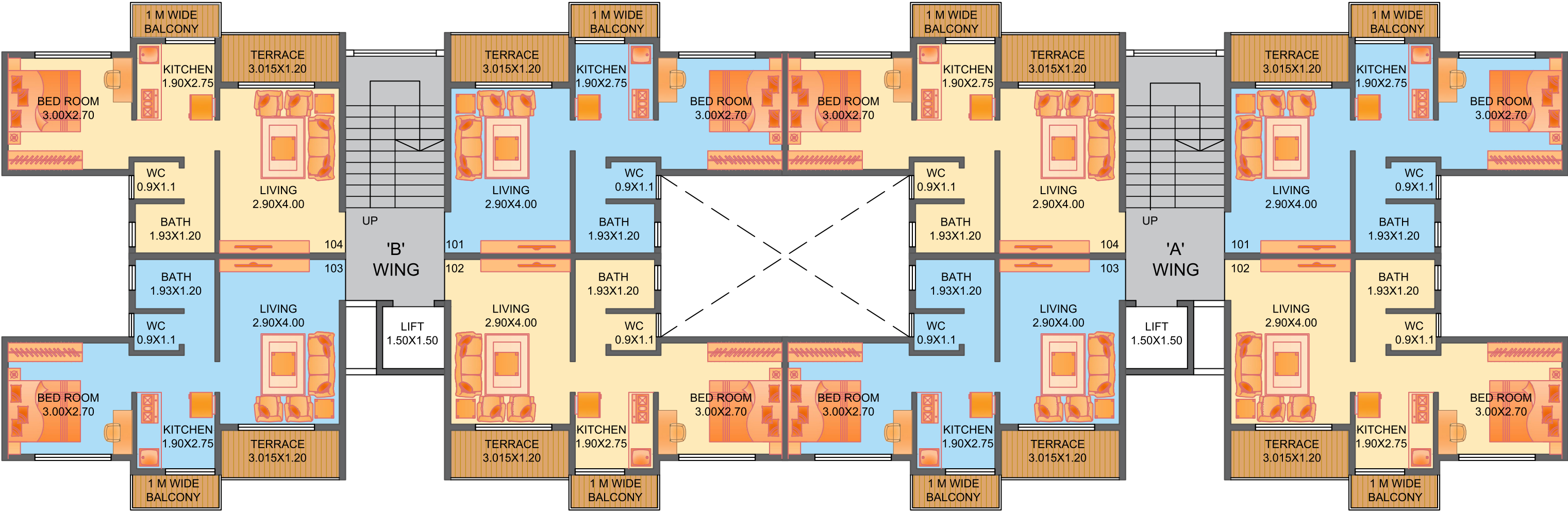
1st ,3rd & 5th FLOOR PLAN
