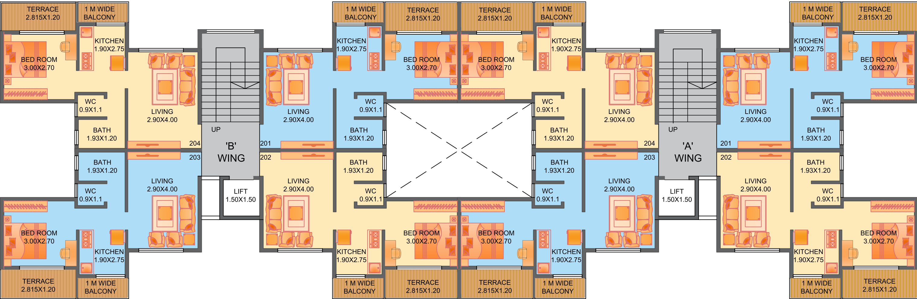
2nd & 4th FLOOR PLAN
